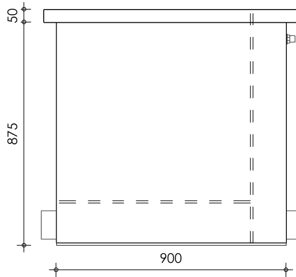
Left-side view
